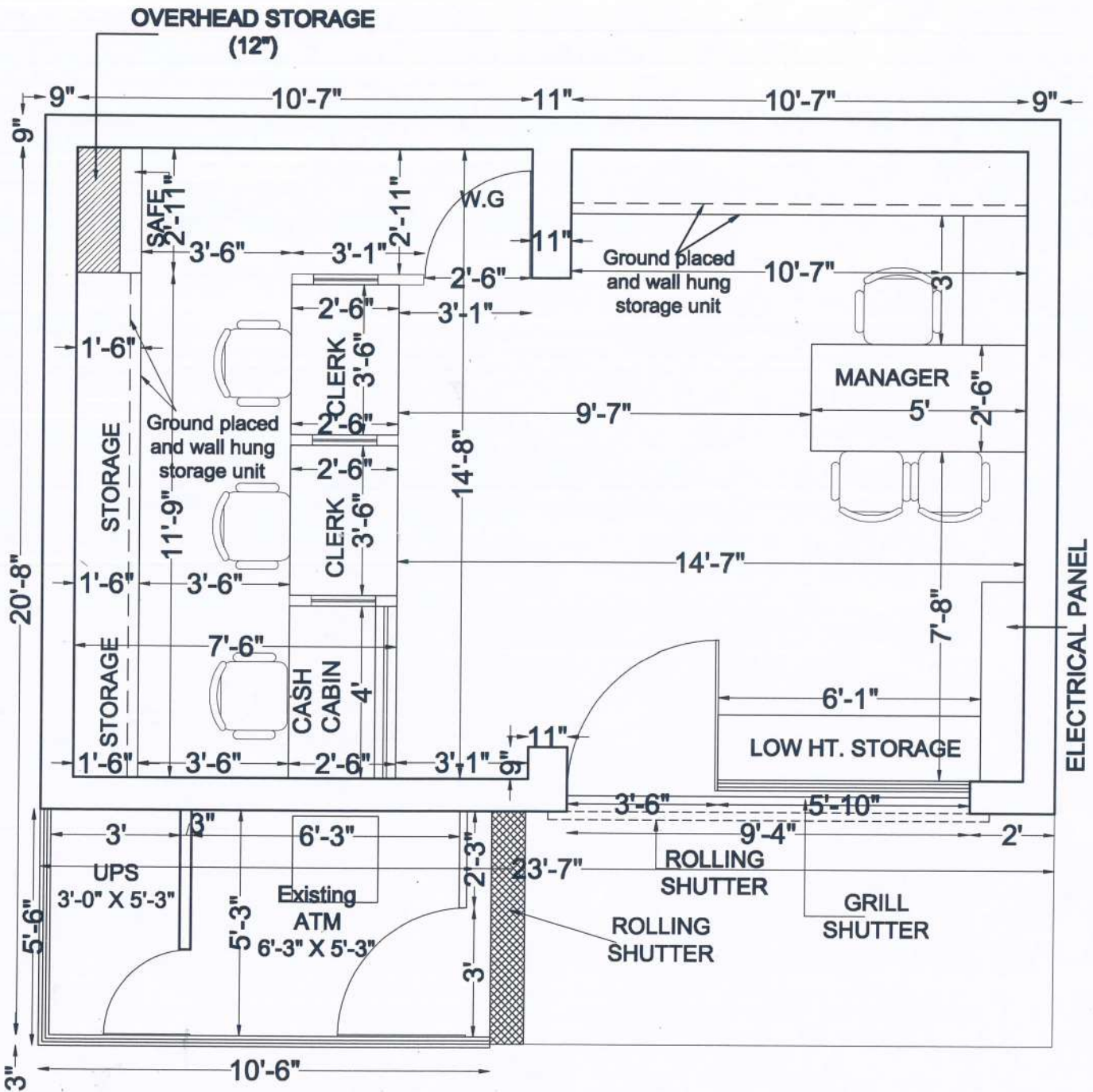
GROUND FLOOR PLAN (REVISED OPTION 1 19-9-2020)
