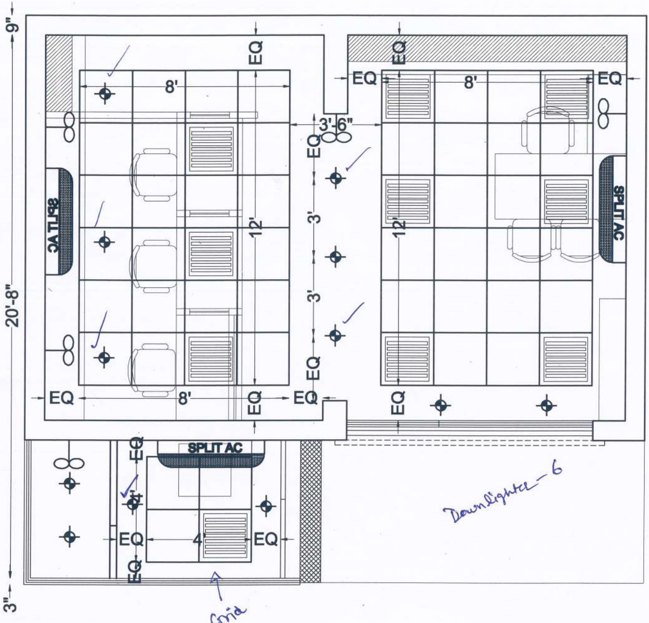
FALSE CEILING PLAN
